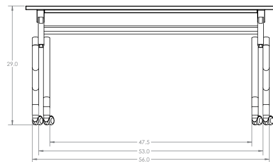
Inside and outside leg spacing for frame for 60" to 72" wide tops.
